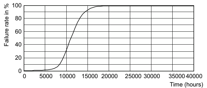
Life Expectancy Diagram - EcoHome LEDBulb 16W E27 6500KHV 1PF/20AR
