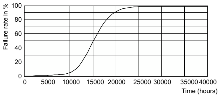
Life Expectancy Diagram - UFO LEDBulb 24W E27 6500K 230V 1CT/6
