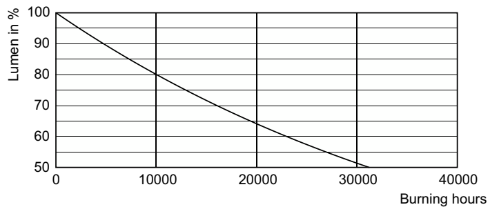
Lumen Maintenance Diagram - UFO LEDBulb 24W E27 6500K 230V 1CT/6
