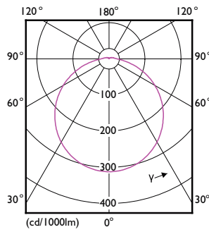
Light Distribution Diagram - UFO LEDBulb 24W E27 6500K 230V 1CT/6
